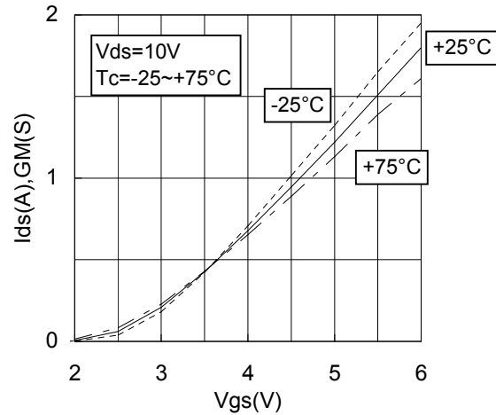
Vgs-Ids CHARACTERISTICS 2
